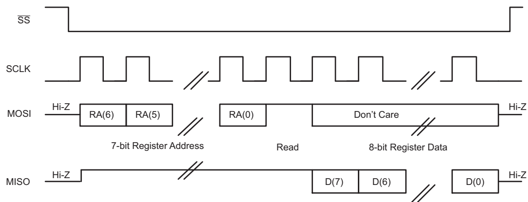
Figure 35. SPI Read
