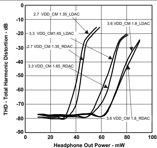
Figure 40. Total Harmonic Distortion vs Headphone Out Power
