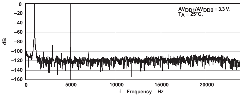
Figure 9. ADC FFT Plot at 48 kps ( T_A = 25^\circ\text{C} , -1 dB, 1 kHz input, AVDD1/AVDD2 = 3.3 V)
