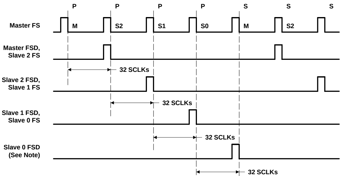
Figure 2–15. Cascade Mode Connection (to DSP Interface)
