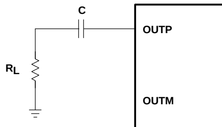
Figure 2–20. Single-Ended Output
