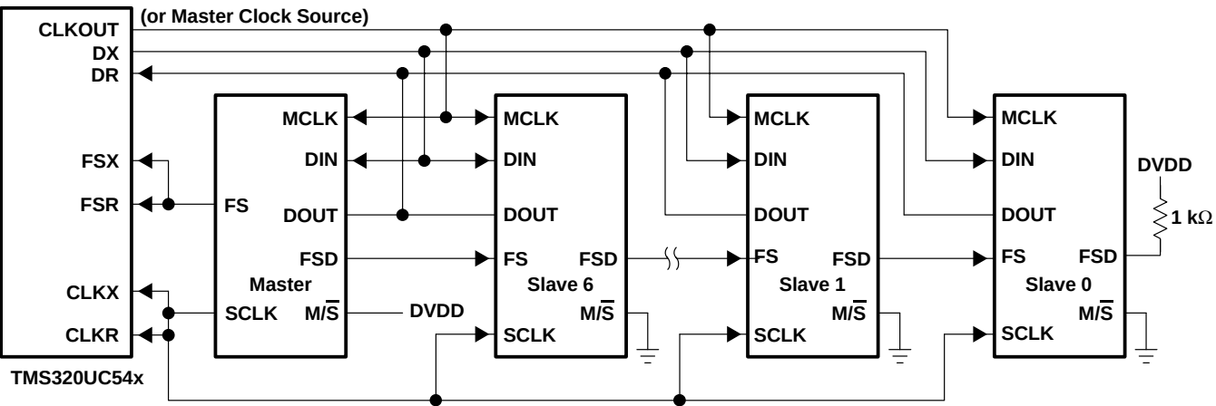
Figure 2-6. Cascading
