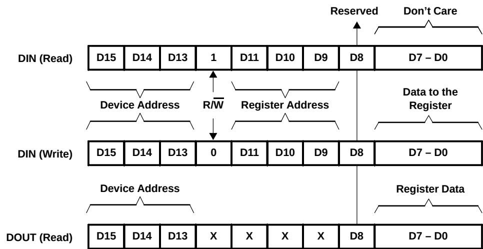
Figure 3-12. Secondary Communication DIN and DOUT Data Format
