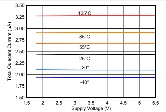
Figure 8-8. Supply Current vs. Supply Voltage
