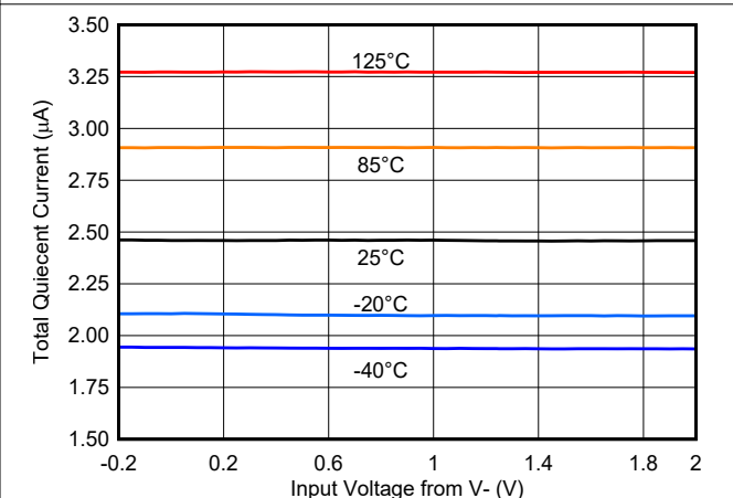
Figure 8-10. Supply Current vs. Common Mode - 1.8V
