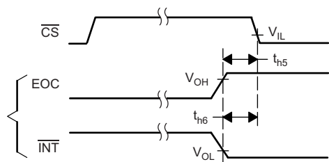
Figure 52. CS and EOC Waveforms
