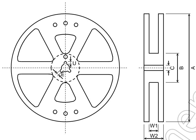
Figure 4 Reel Form
