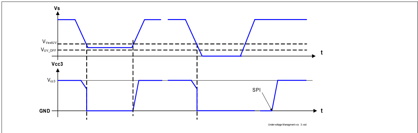
Figure 9 Supply Voltage Management
