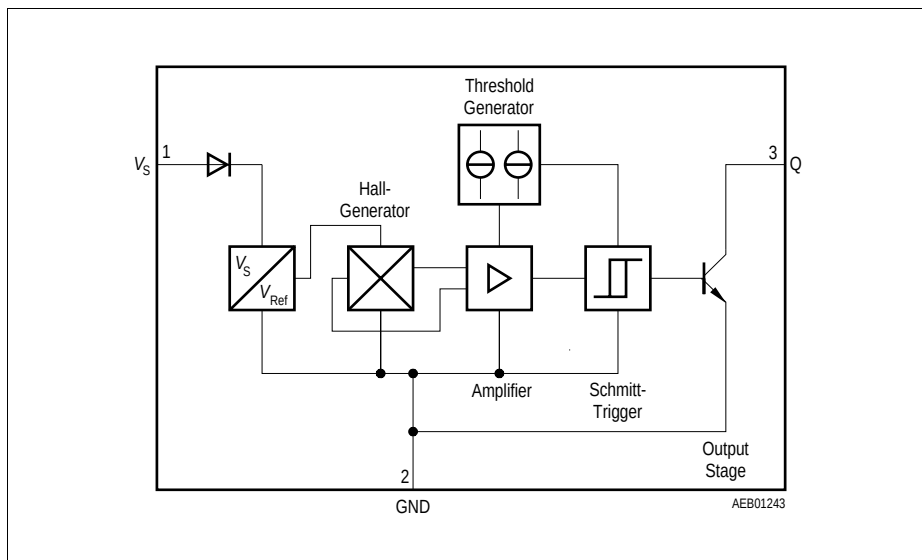
Figure 2 Block Diagram
