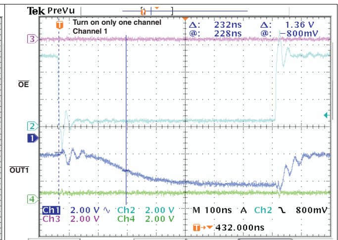
Figure 2. Response Time, \overline{OE} to OUT_1
