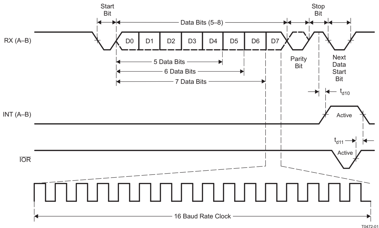
Figure 15. Receive Timing
