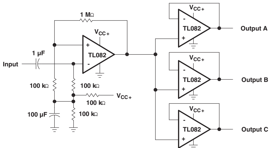
Figure 22. Audio-Distribution Amplifier
