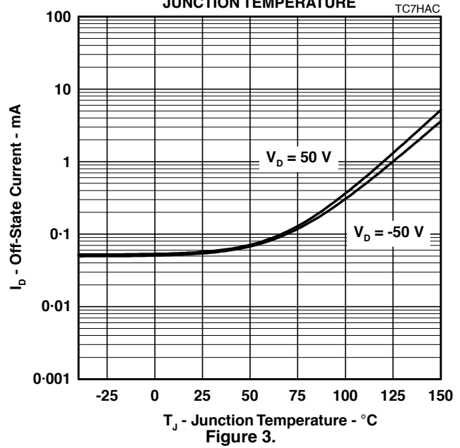
TISP7240F3 THRU TISP7380F3 OFF-STATE CURRENT vs JUNCTION TEMPERATURE
