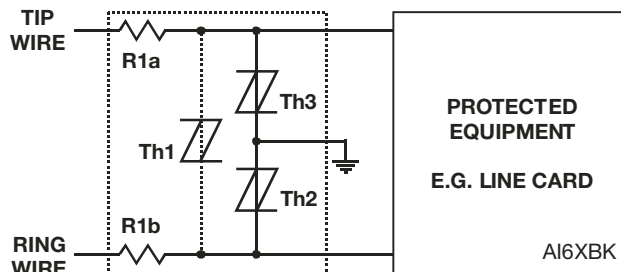
Figure 16. PROTECTION MODULE
