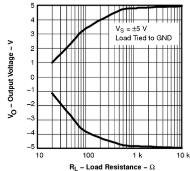
Figure 8. Output Voltage vs Load Resistance
