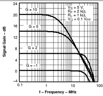
Figure 19. Frequency Response
