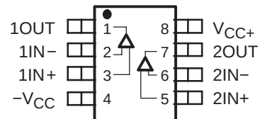
THS4052 D AND DGN† PACKAGES (TOP VIEW)
