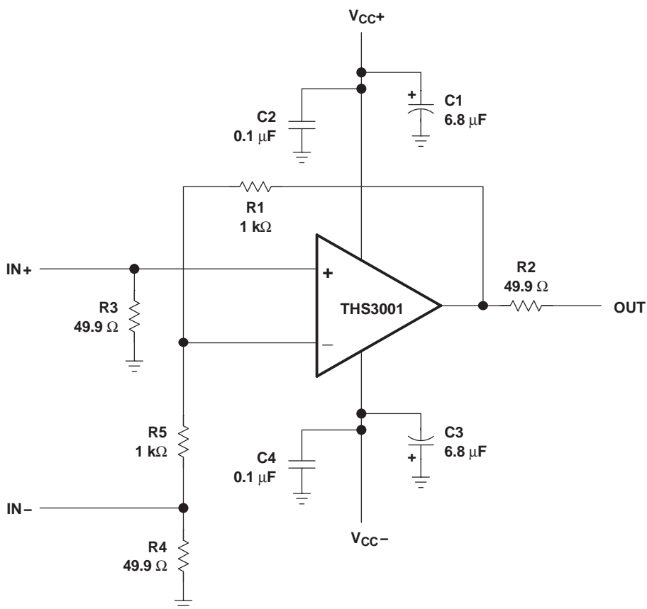
Figure 61. THS3001 Evaluation Board Schematic
