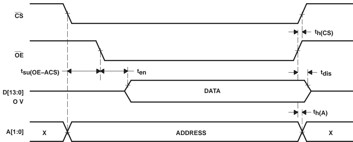
Figure 2. Read Timing
