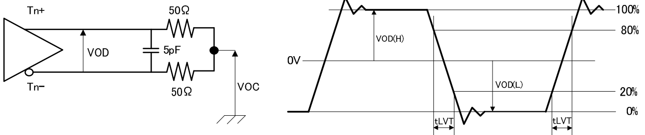
Figure 6. LVDS Output Load and Transition Time
