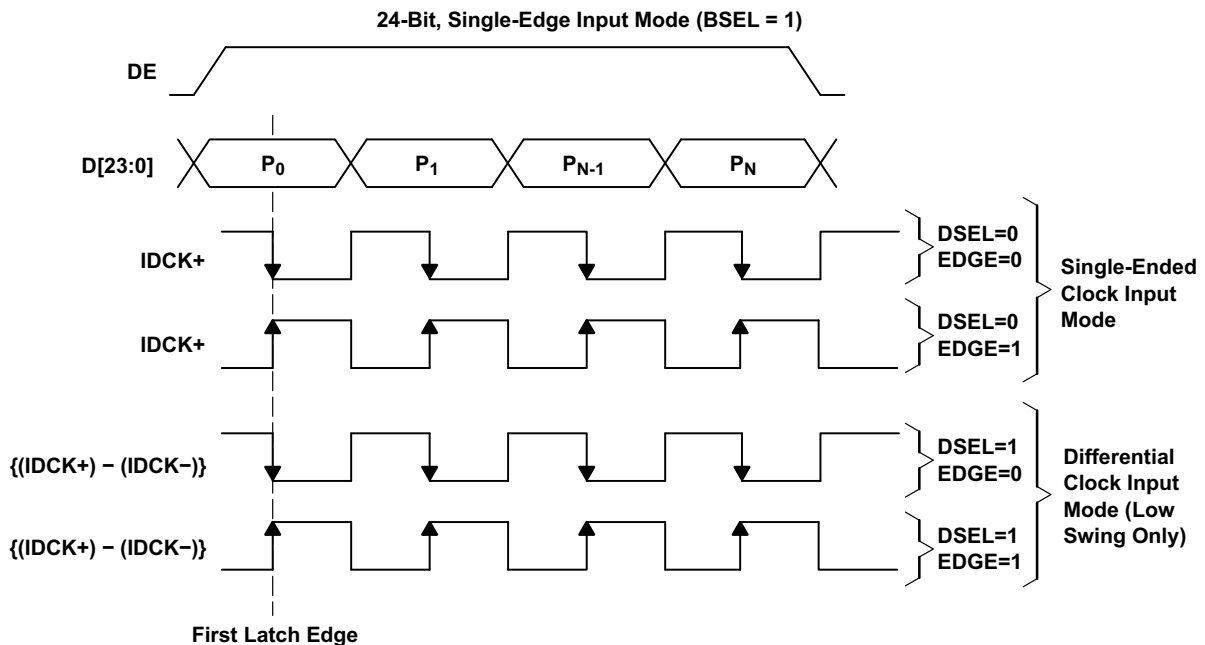
Figure 6-2. Universal Graphics Controller Interface Options for 24-Bit Mode (Graphical Representation)
