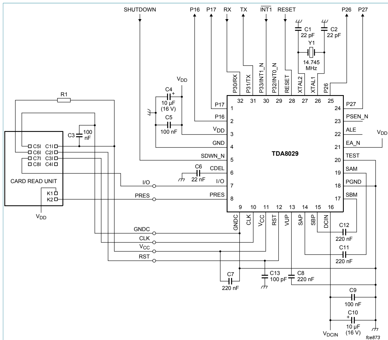
Figure 14. Application diagram
