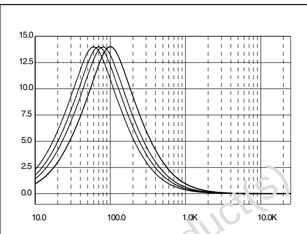
Figure 13. Bass normal and DC mode @ Gain = 14 dB, f_c = 80 Hz (1)
