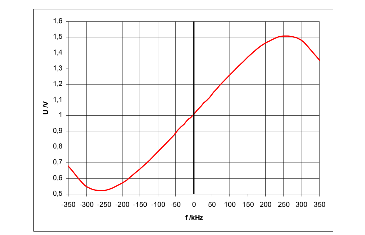
Figure 2-4 Quadratic Demodulation Characteristic
