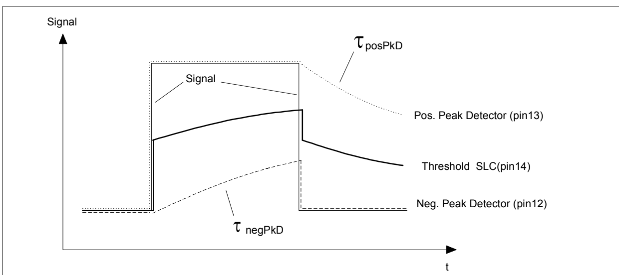
PkD_timing.wmf
