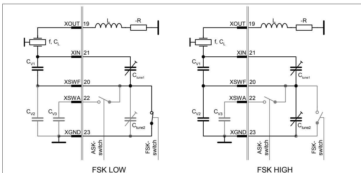
Figure 3-17 FSK modulation
