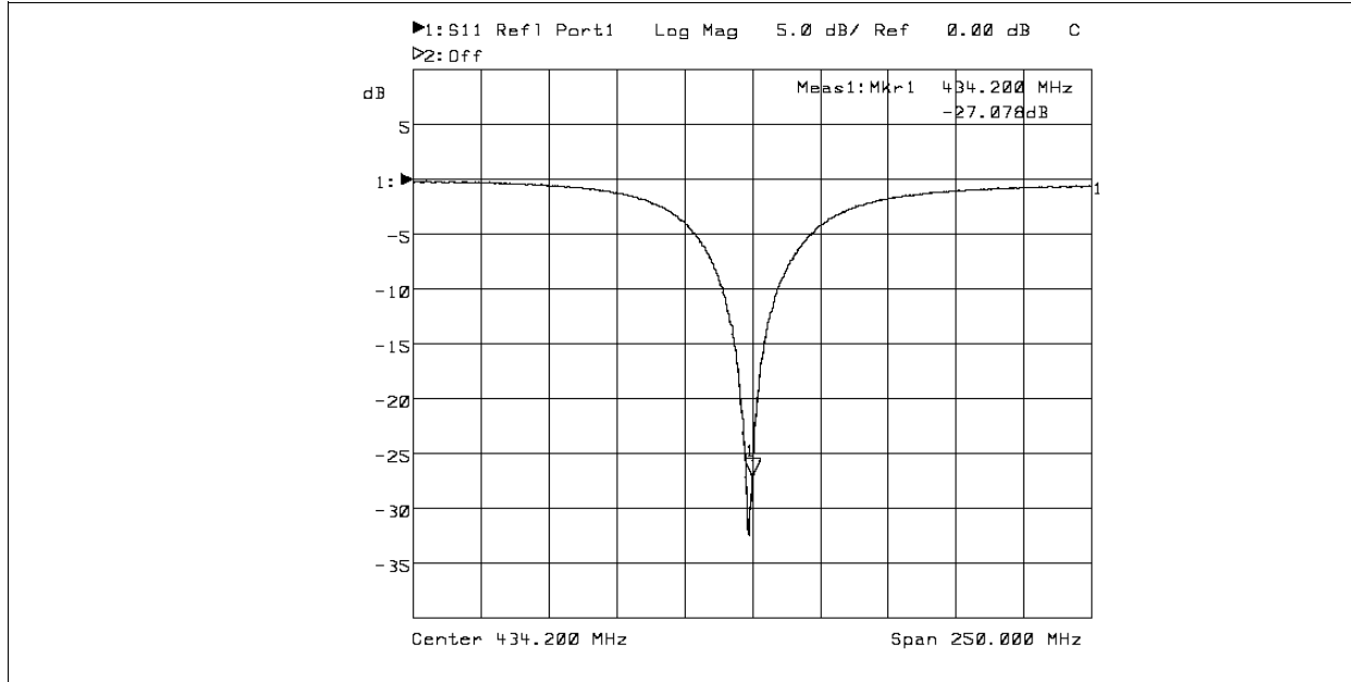
Figure 3-3 S11 measured
