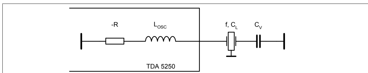
Figure 3-15 Crystal Oscillator
