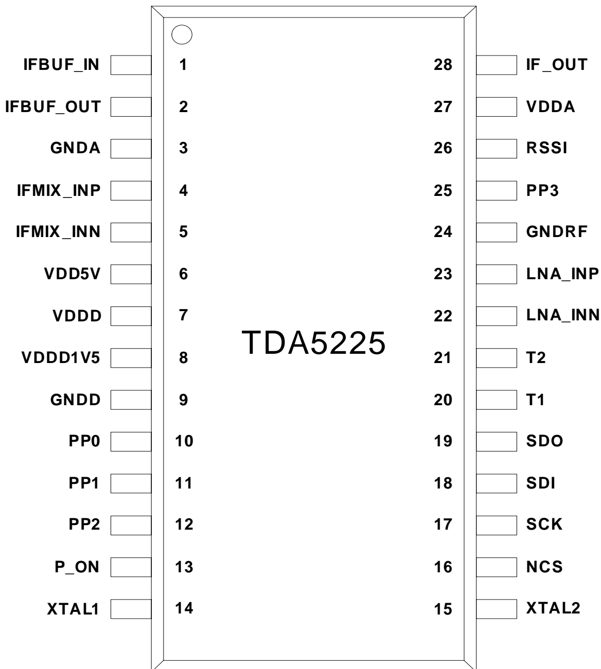
Figure 1 Pin-out
