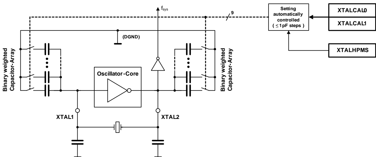
Figure 7 Crystal Oscillator
