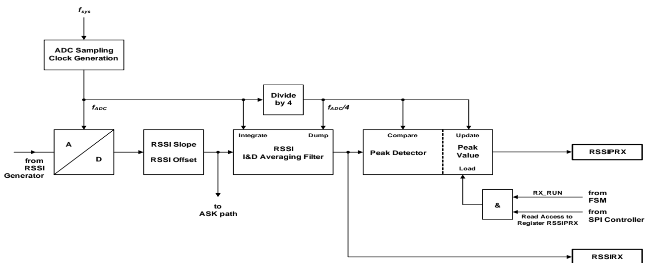
Figure 13 Peak Detector Unit
