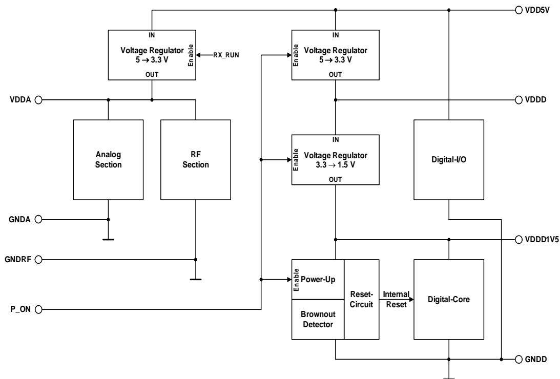
Figure 18 Power Supply
