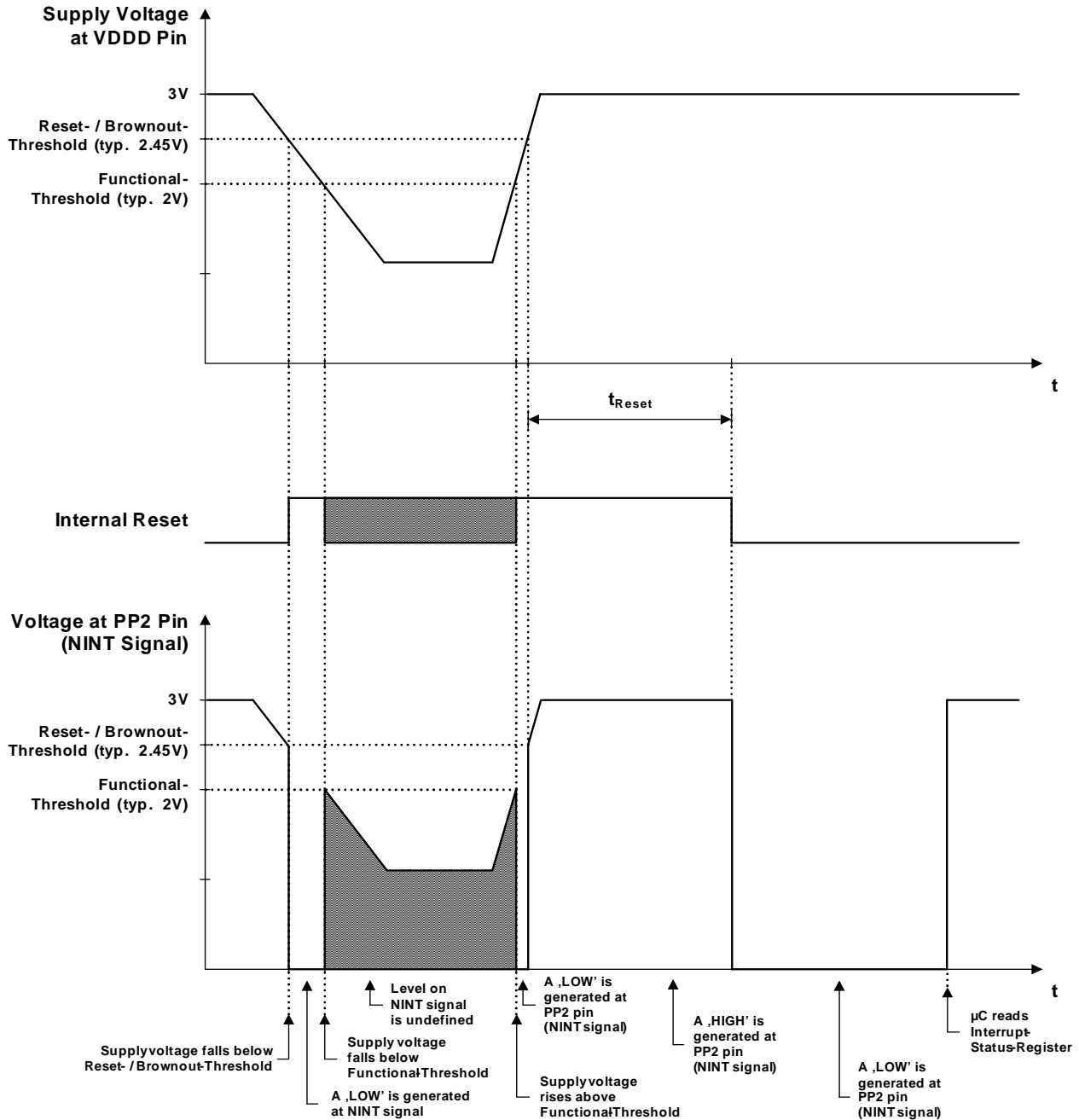
Figure 21 Reset Behavior
