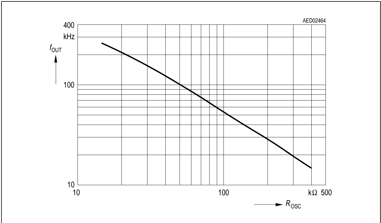
Figure 5 PFC/PWM Frequency
