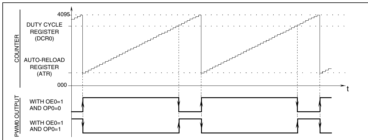
Figure 35. PWM Function
