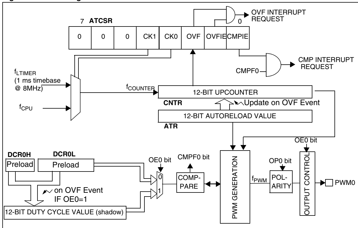
Figure 34. Block Diagram
