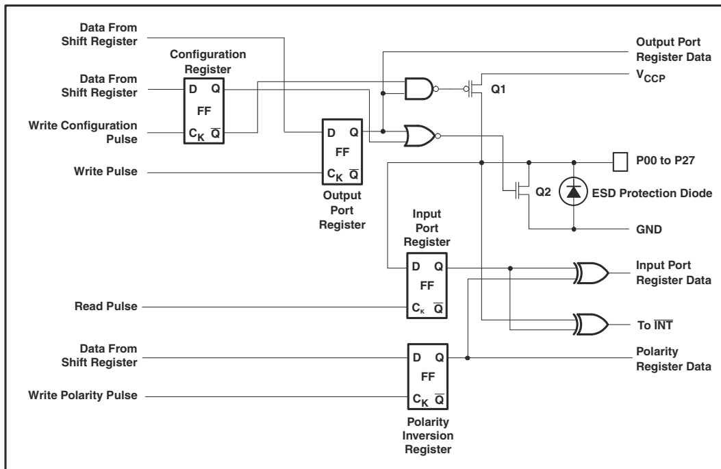
Figure 8-1. Positive Logic
