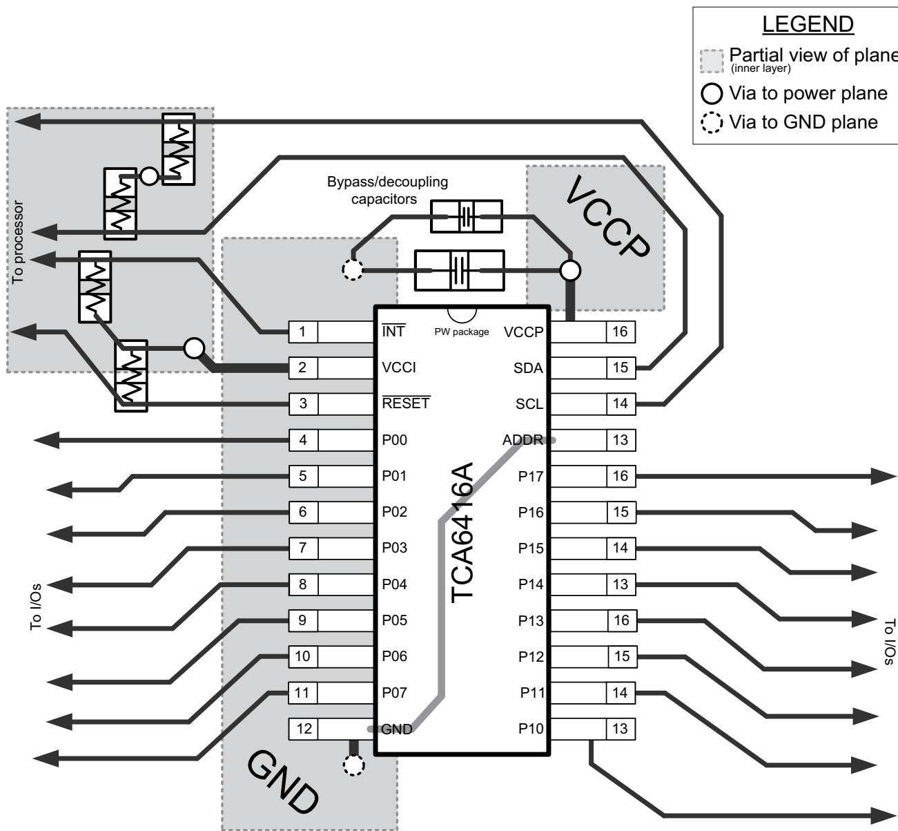
Figure 11-1. TCA6416A Layout
