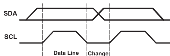
Figure 25. Bit Transfer
