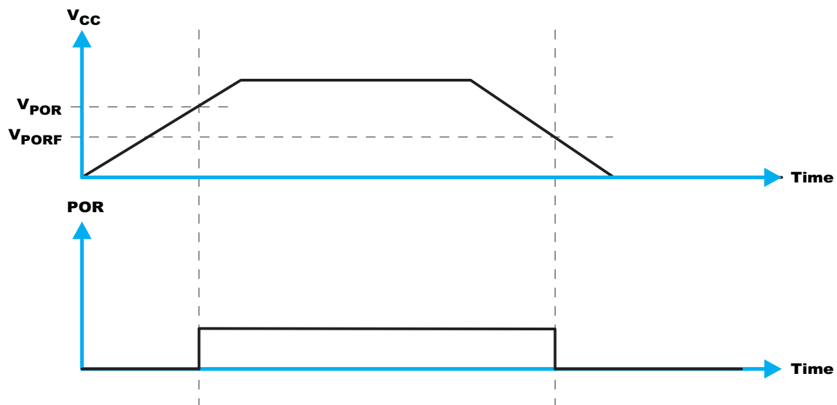
Figure 41. V_{POR}
