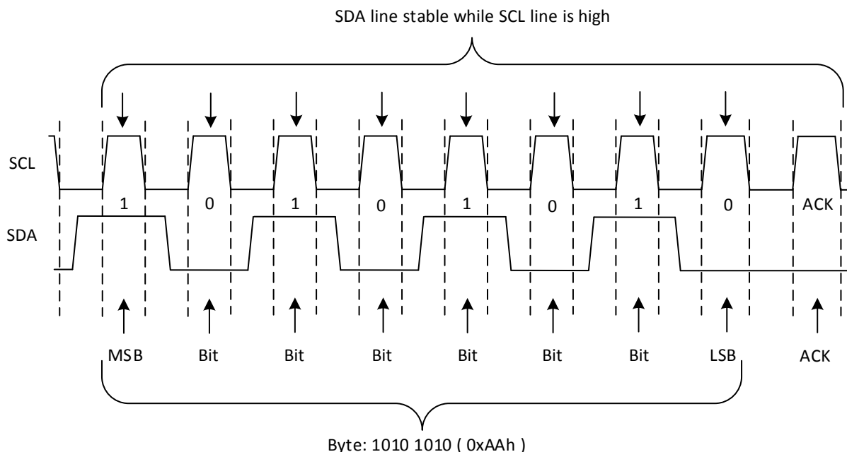
Figure 8-4. Bit Transfer
