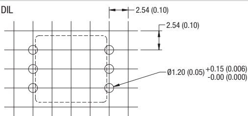
6 Pin DIL
