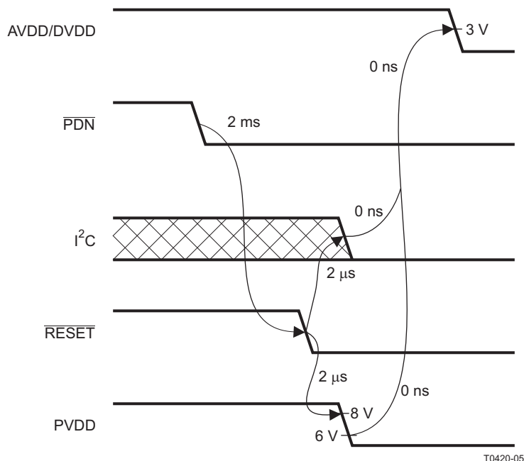
Figure 42. Power-Loss Sequence
