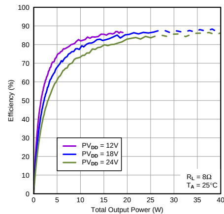
Figure 44. Efficiency vs Total Output Power
