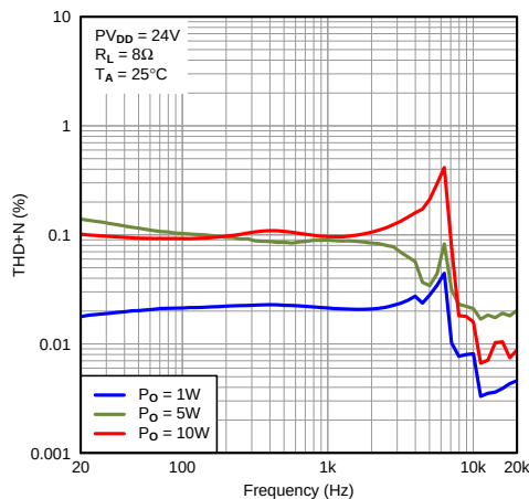
Figure 43. Total Harmonic Distortion + Noise vs Frequency
