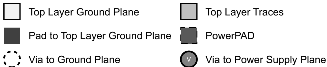
Figure 82. Layout Recommendation
