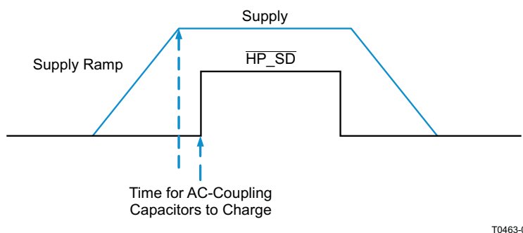
Figure 50. Power-Up/Down Sequence
