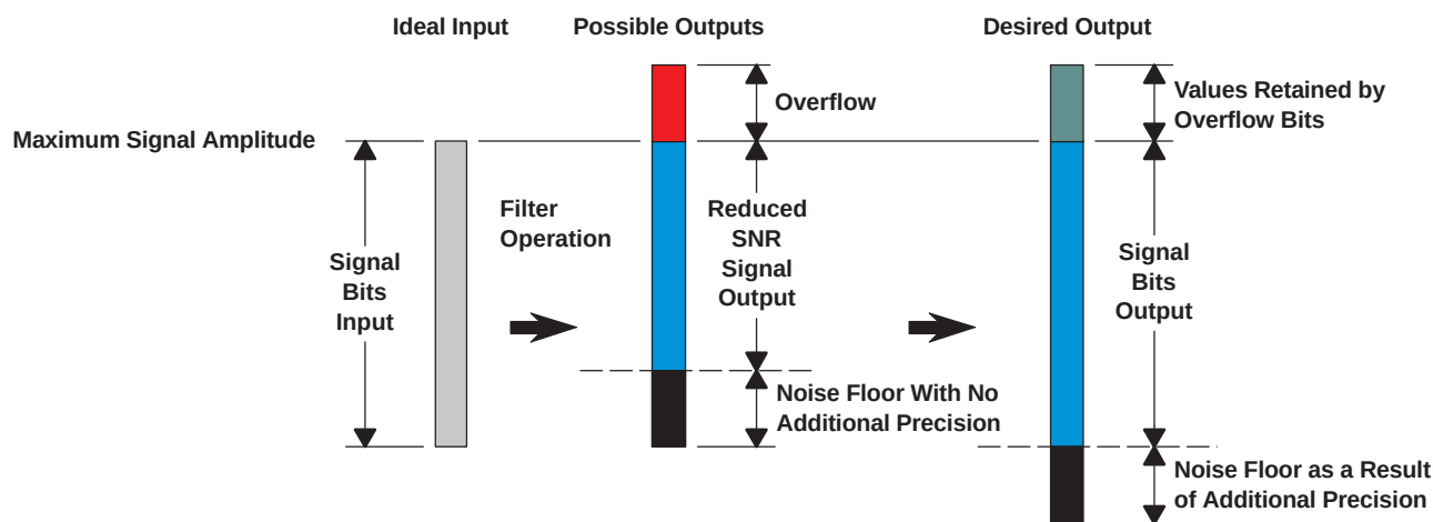
Figure 2-10. TAS5508C Digital Audio Processing
