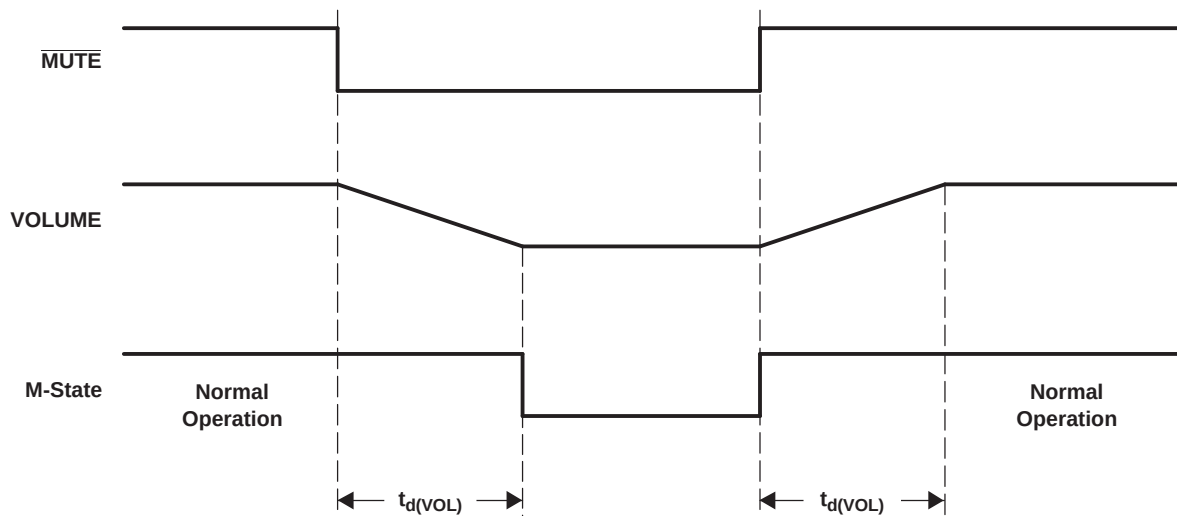
Figure 4-7. Mute Timing
