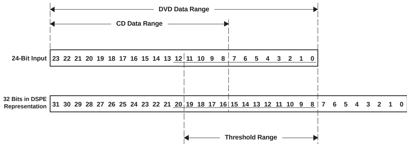
Figure 2-13. Automute Threshold
