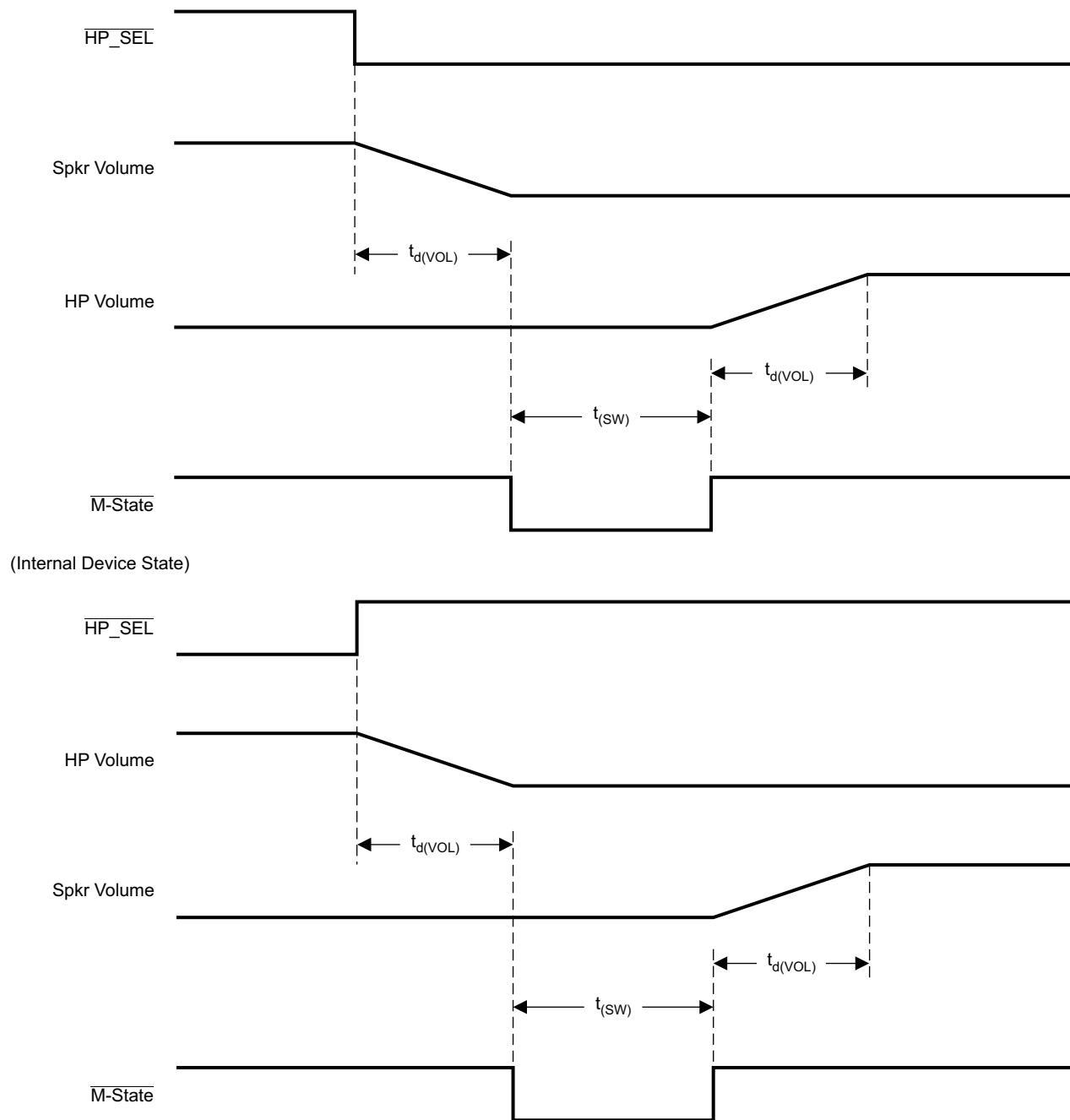
Figure 4-8. \overline{\text{HP\_SEL}} Timing
