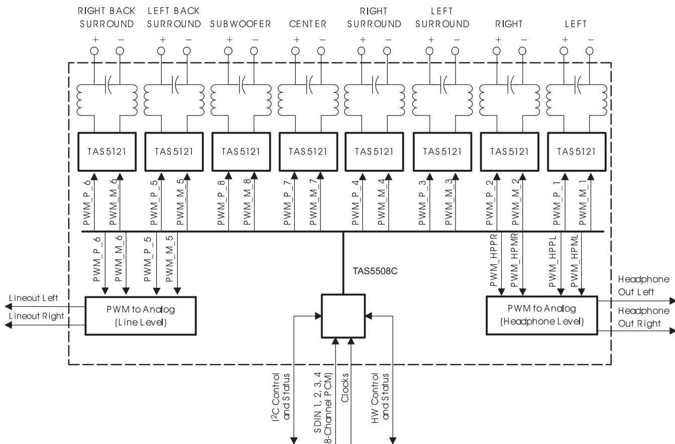
Figure 1-3. Recommended TAS5508C and TAS5121 Channel Configuration
