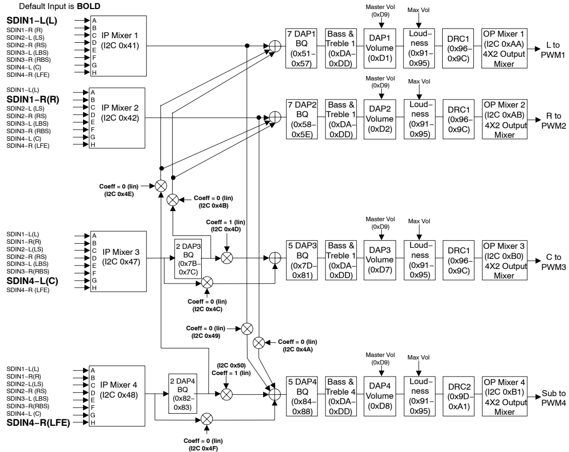
Figure 1-2. TAS5504 DAP Architecture With I 2 C Registers (Fs ≤ 96 kHz)
