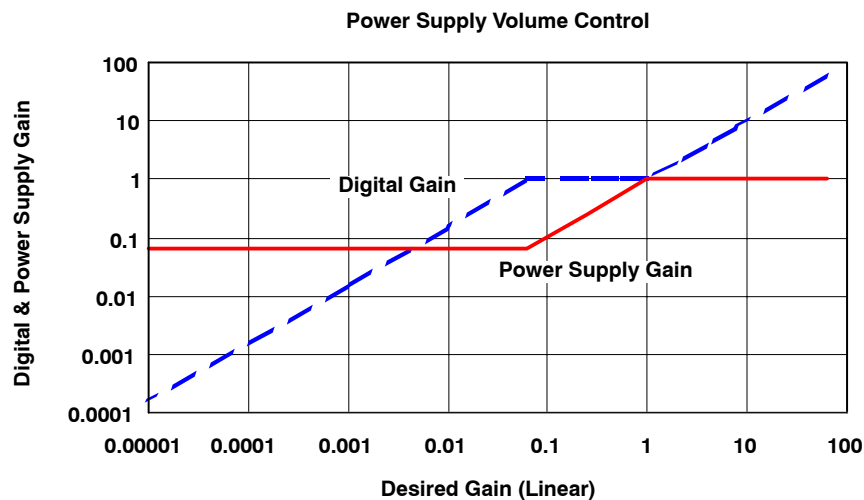
Figure 1-23. Power Supply and Digital Gains (Linear Space)
