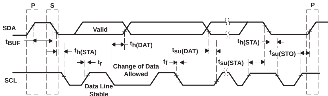
Figure 3-4. I 2 C Serial Port Timing
