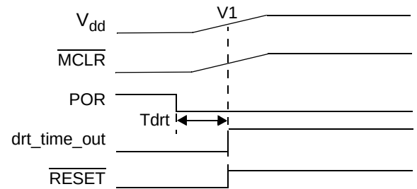
Figure 12-3. Time-out Sequence on Power-up ( \overline{\text{MCLR}} tied to V_{dd} ): Slow Rise Time
