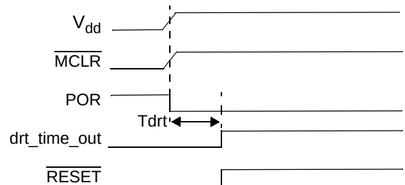
Figure 12-5. Time-out Sequence on Power-up ( \overline{\text{MCLR}} tied to V_{dd} ): Fast V_{dd} Rise Time
