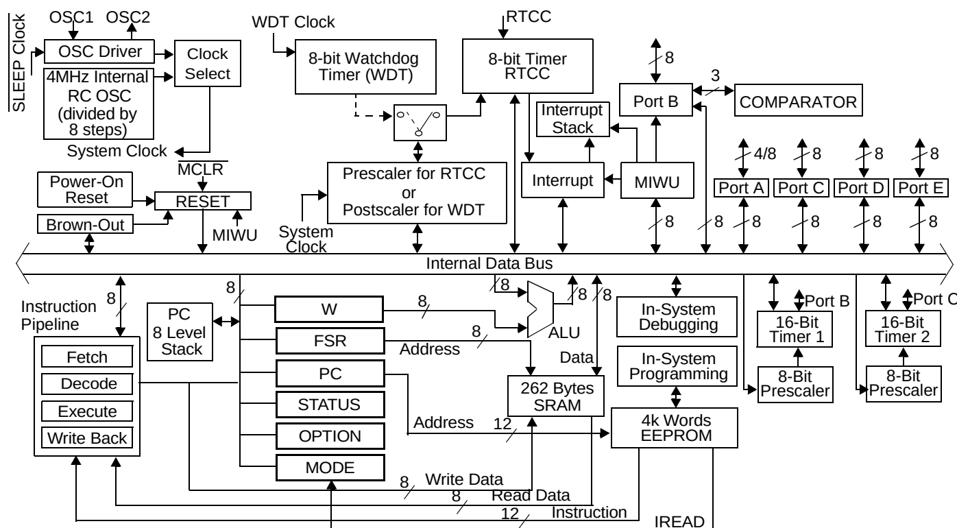
Figure 1-1. Block Diagram
