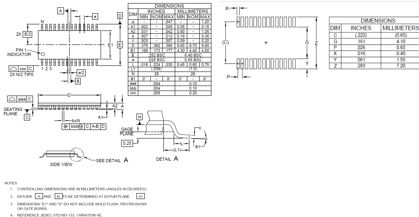
Figure 44. TSSOP 28 Package Outline Drawing and Land Pattern
