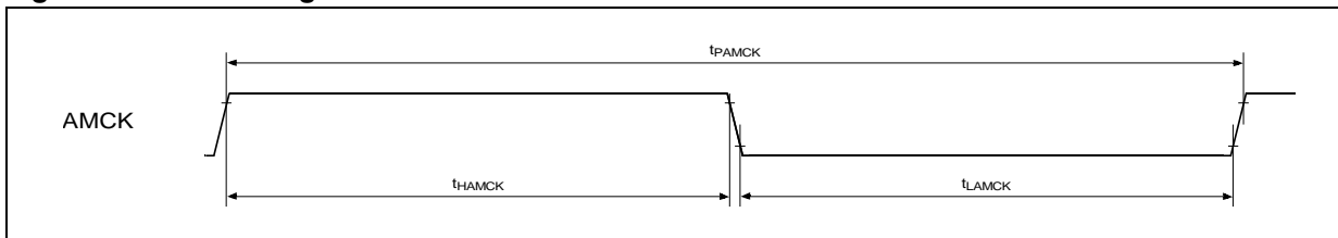
Figure 4. AMCK timing
