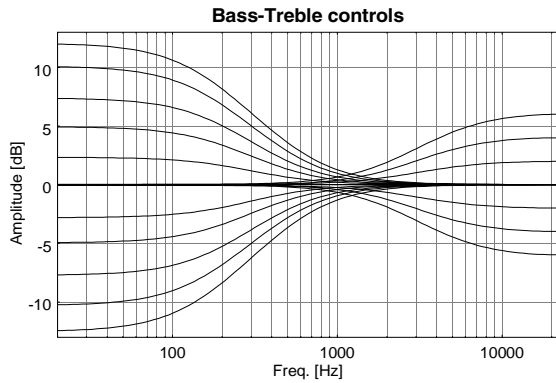
Plot 1. Bass and treble gains are independently selectable in any combination. Filters characteristics at F_s=44.1\text{kHz} are plotted
