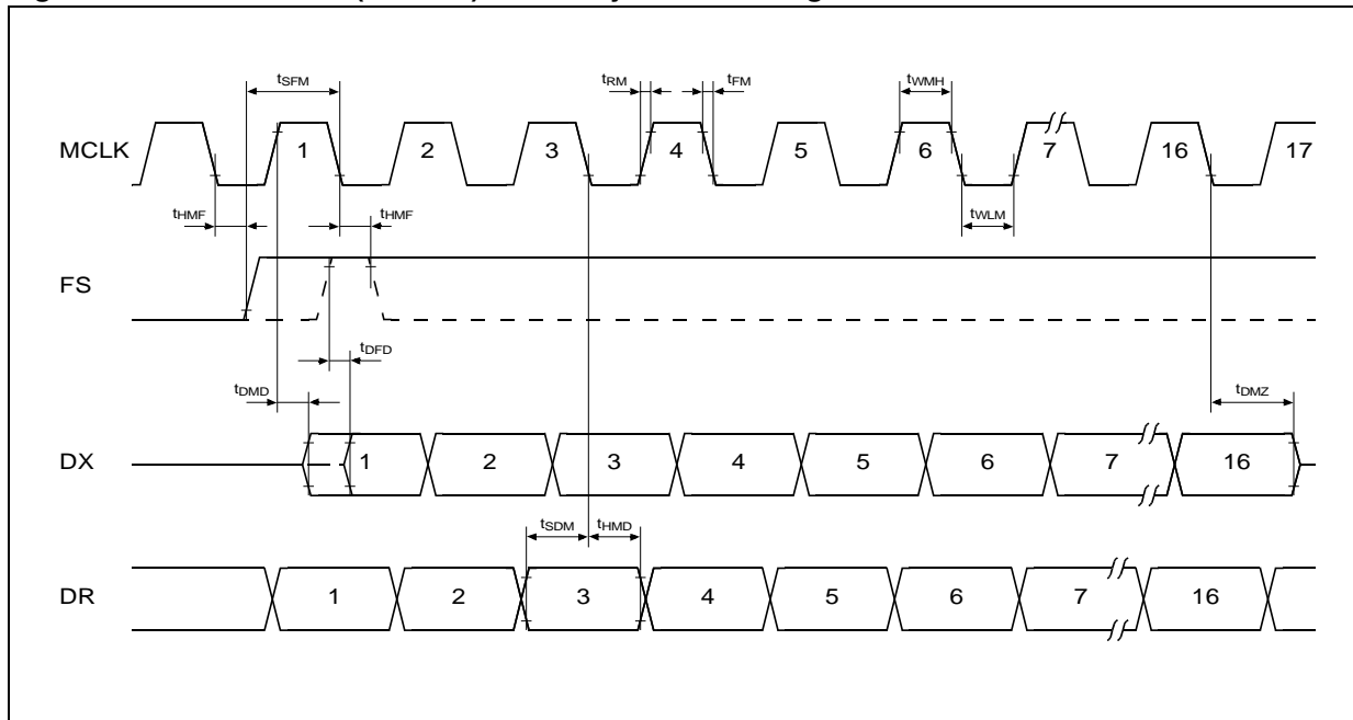
Figure 1. Voice interface (PCM I/F) non delayed data timing mode 1
