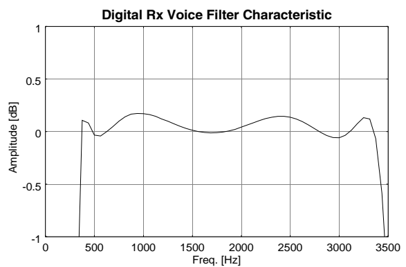
Plot 6. In band Frequency response. F_s=8\text{ kHz}
