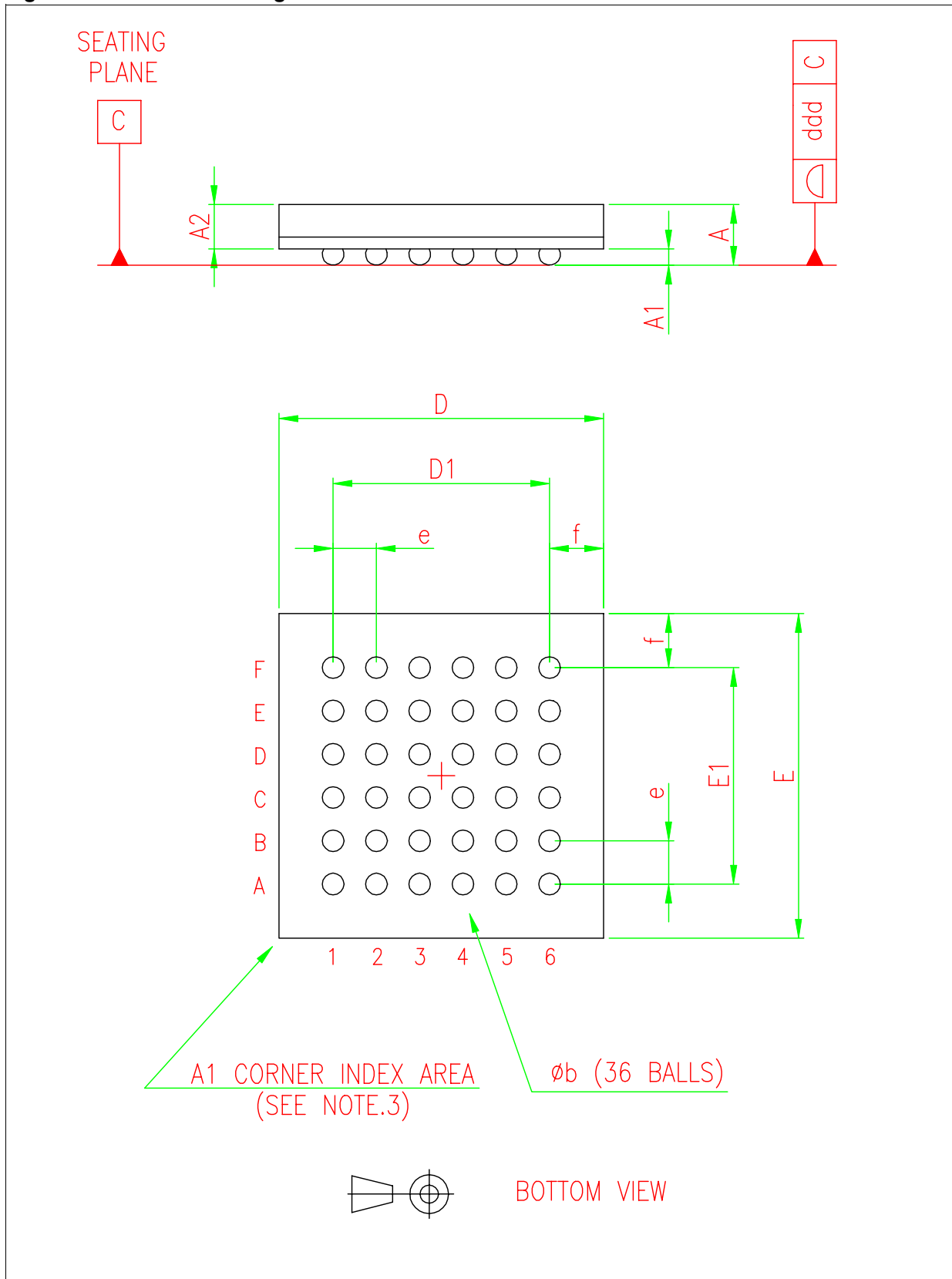
Figure 17. TFBGA36 drawing
