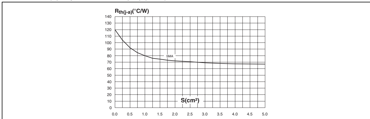
Figure 15. Thermal resistance junction to ambient versus copper surface under each lead (epoxy FR4, Cu = 35 \mu\text{m} ) (SMA)
