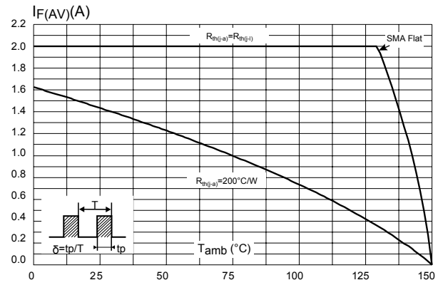
Figure 4. Average forward current versus ambient temperature ( \delta = 0.5 , SMA Flat)
