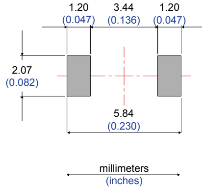
Figure 21. Footprint recommendations, dimensions in mm (inches)
