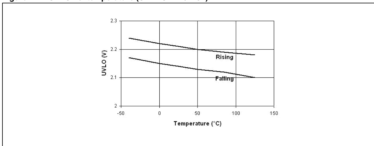
Figure 27. UVLO vs. temperature (STMP2141/2151)
