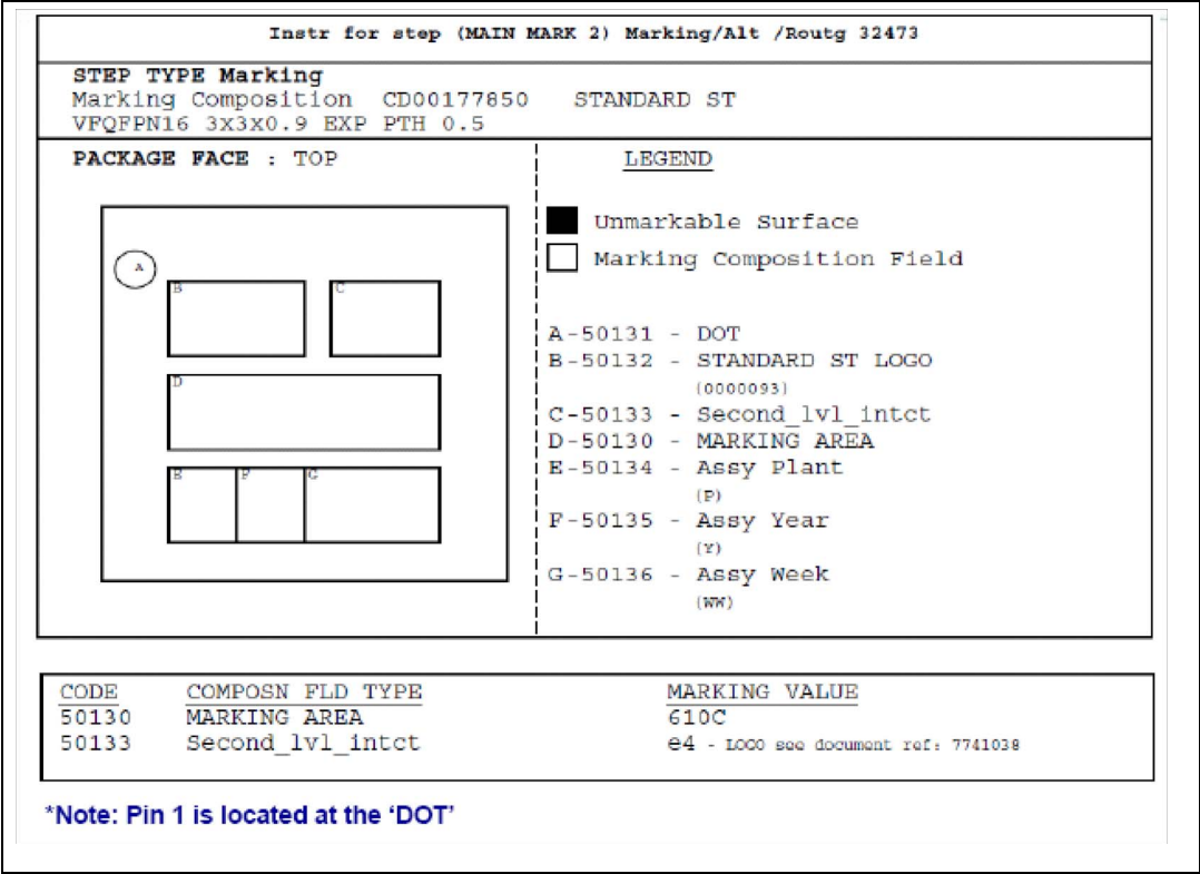
Figure 17. Marking specifications
