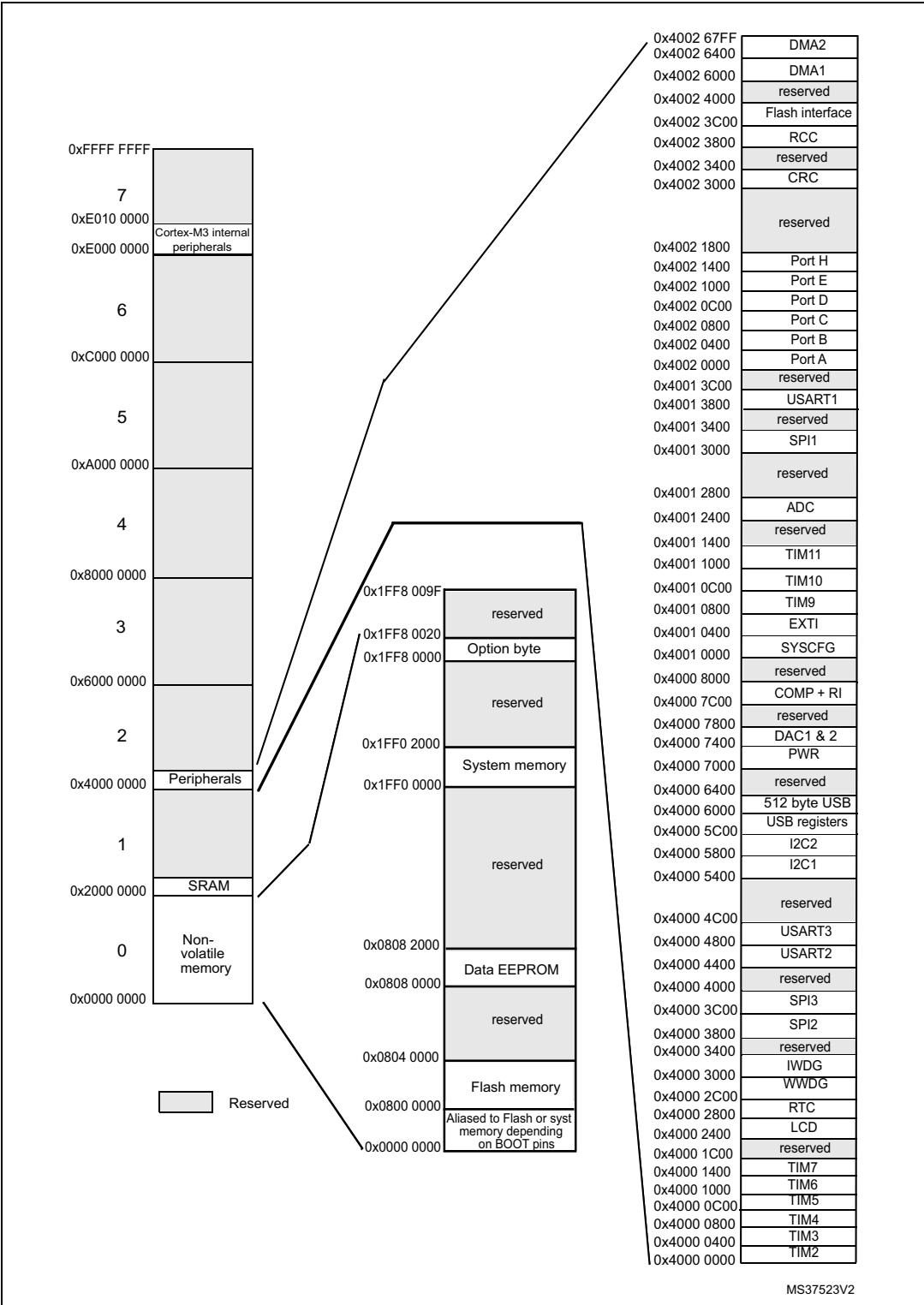
Figure 8. Memory map
