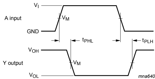
Figure 8. The data input (A) to output (Y) propagation delays
