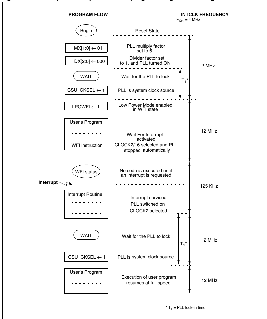
Figure 64. Example of low power mode programming in WFI using CLOCK2/16
