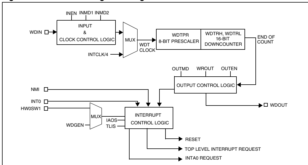
Figure 85. Timer/watchdog block diagram
