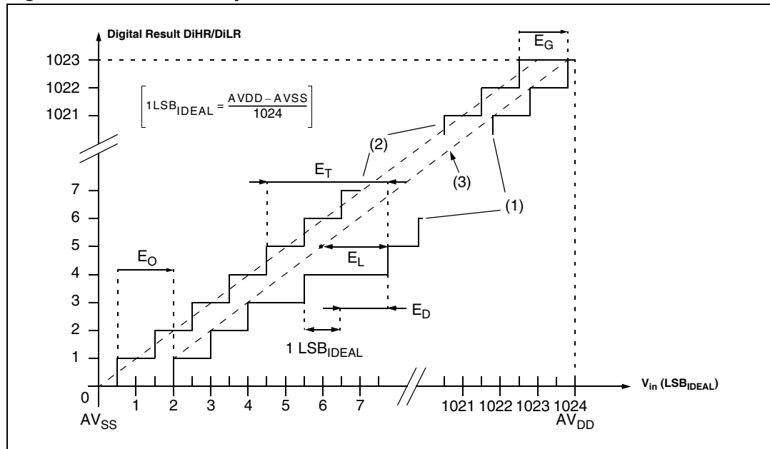
Figure 196. ADC accuracy characteristics
