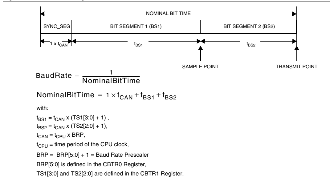
Figure 166. Bit timing
