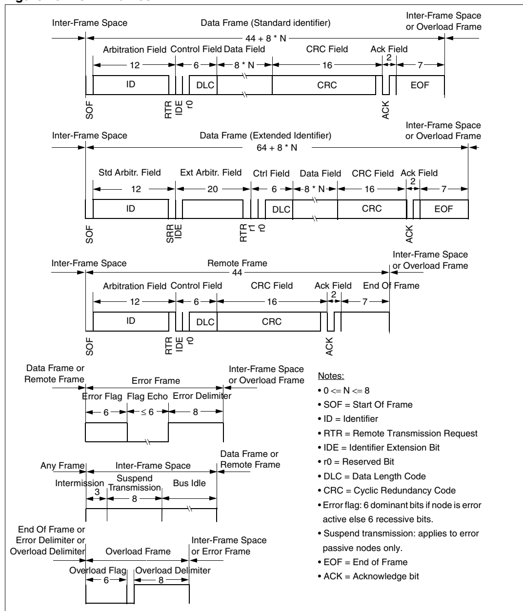
Figure 167. CAN frames
