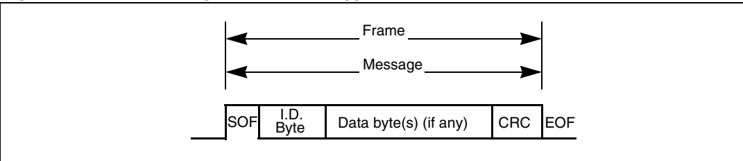
Figure 144. J1850 string transmission type 0
