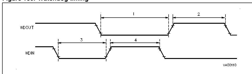
Figure 180. Watchdog timing
