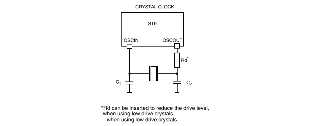
Figure 66. Crystal oscillator
