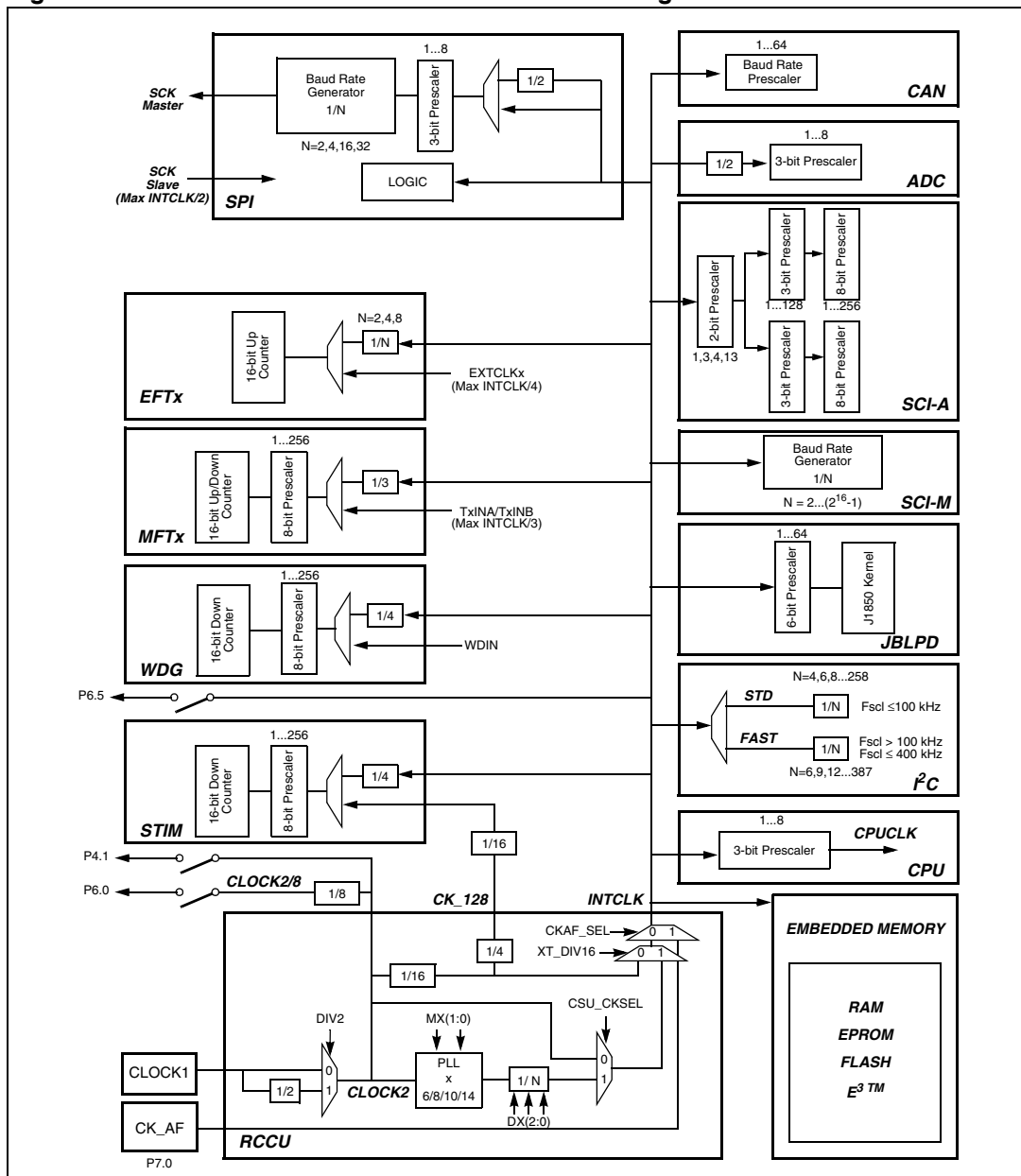
Figure 60. ST92F124/F150/F250 clock distribution diagram
