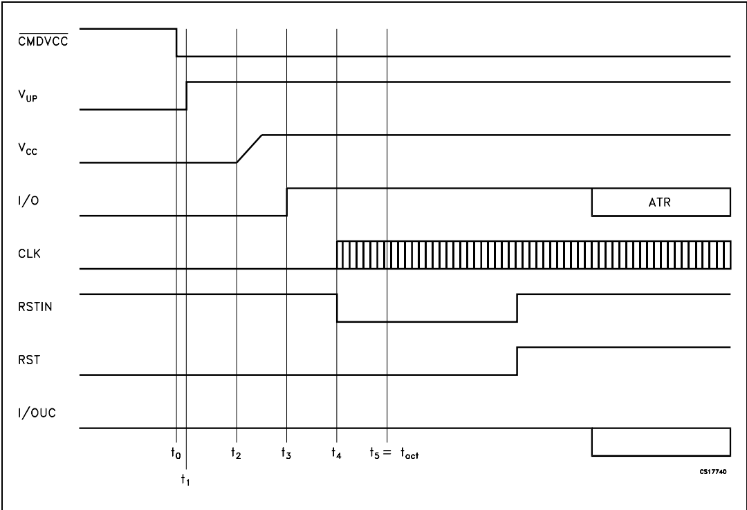
Figure 5. Activation sequence using RSTIN and CMDVCC
