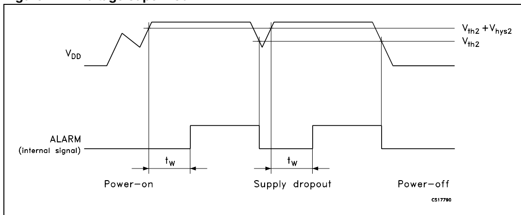
Figure 4. Voltage supervisor
