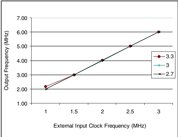
Figure 57. PLLx4 Output vs CLKIN frequency
