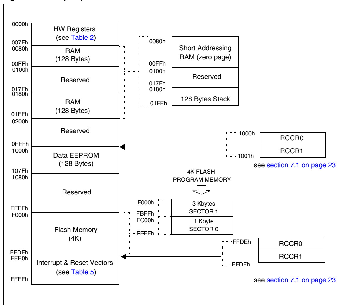
Figure 3. Memory Map
