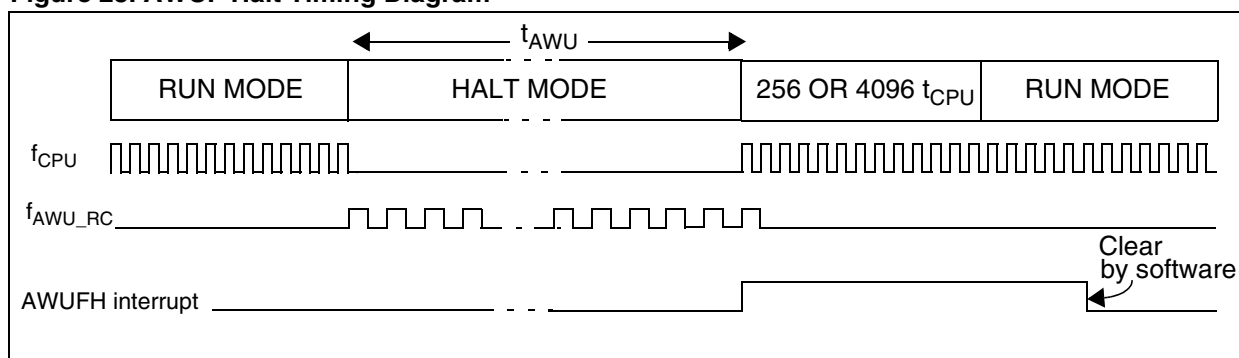
Figure 28. AWUFH Halt Timing Diagram
