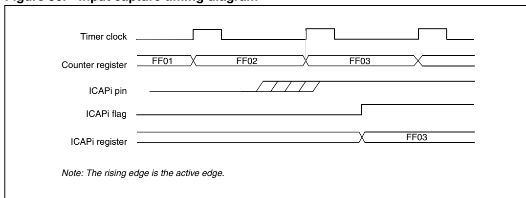
Figure 30. Input capture timing diagram
