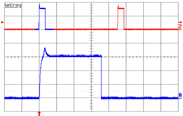
Figure 15. Load current (top trace, 20 A/div., 50 ms/div.) into a 10 ms short circuit during restart, at V_{in} = 48 V. Bottom trace (10 A/div., 5 ms/div.) is an expansion of the on-time portion of the top trace
